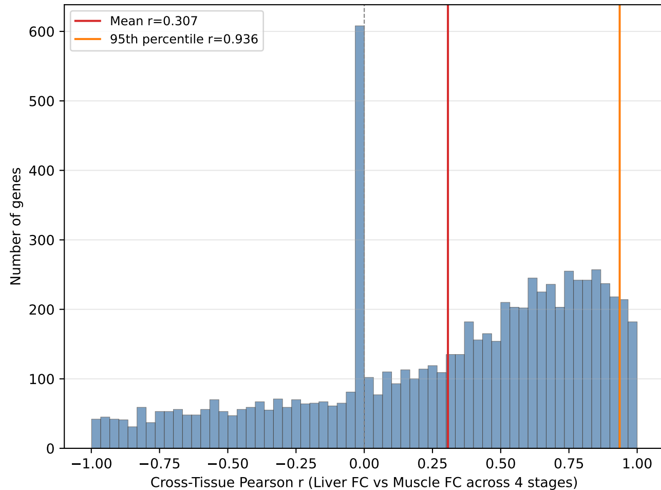
Distribution of Cross-Tissue FC Correlations (n=7464 common genes)
