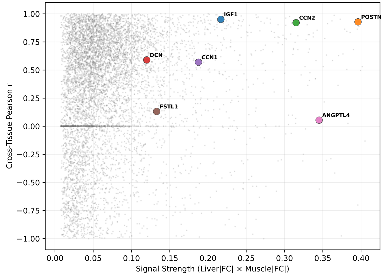
Cross-Tissue Coordination vs Signal Strength (Hepatokines labeled)
