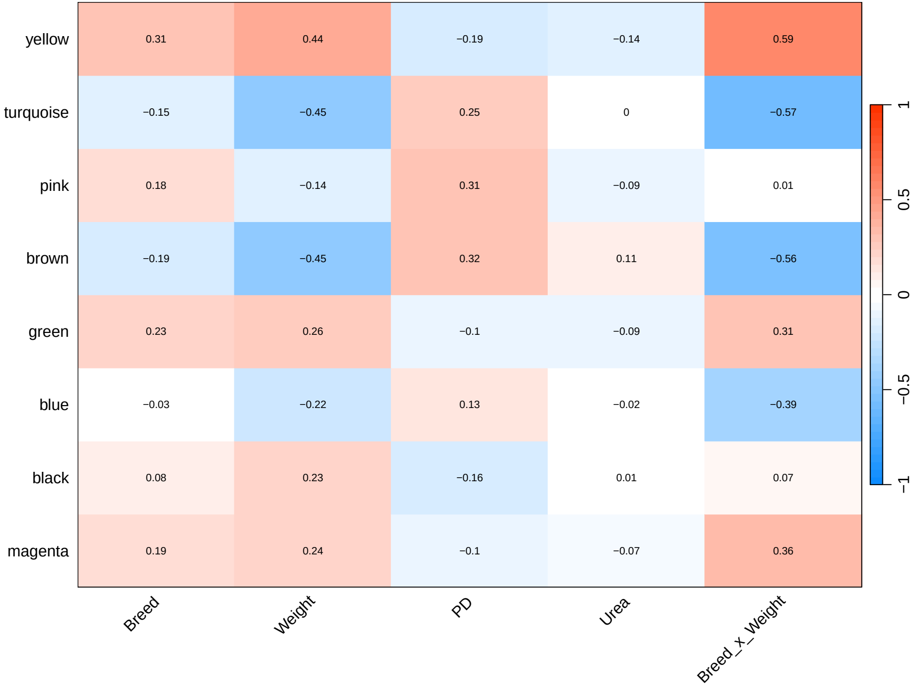
Liver Module–Trait Correlations
