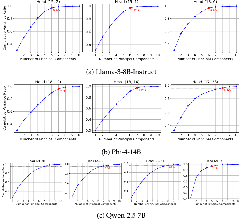
Figure 4: Cumulative explained variance ratio vs. number of PCs for each main head. The first six PCs capture 97% of the task variance for the Llama-3-8B-Instruct main heads; the Phi-4 main heads reach 95% at 7–8 PCs and the Qwen-2.5-7B main heads at 5–8 PCs.
