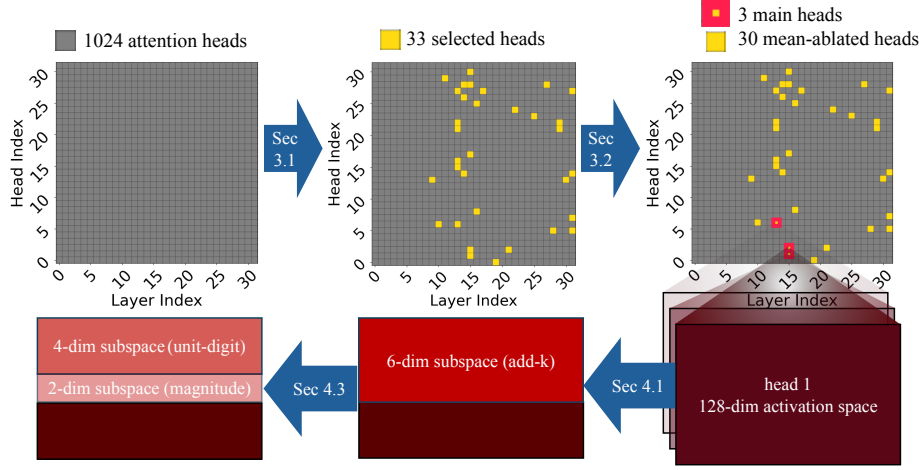
Figure 2: The chain of localization in §3 and §4. We first select 33 attention heads (out of 1024) via a global optimization method (§3.1), then narrow down to 3 main heads while mean-ablating the remaining 30 (§3.2). We next study the structure of the representation of each main head by localizing it to a six-dimensional subspace (§4.1), and decompose it into a four-dimensional subspace encoding the units digit and a two-dimensional subspace encoding the coarse magnitude (i.e., the tens digit) (§4.3).
