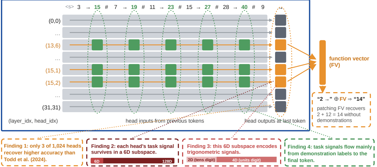
Figure 1: Key findings illustrated on Llama-3-8B-Instruct and a five-shot add-12 prompt as an example: (1) only three attention heads carry most of the add-k task signal (§3); (2) each head’s signal survives in a six-dimensional subspace of its outputs (§4.1); (3) that subspace trigonometrically encodes k with four dimensions for the units digit and two dimensions for the tens digit (§4.2, §4.3); and (4) signals flow mainly from demonstration labels (§5).
