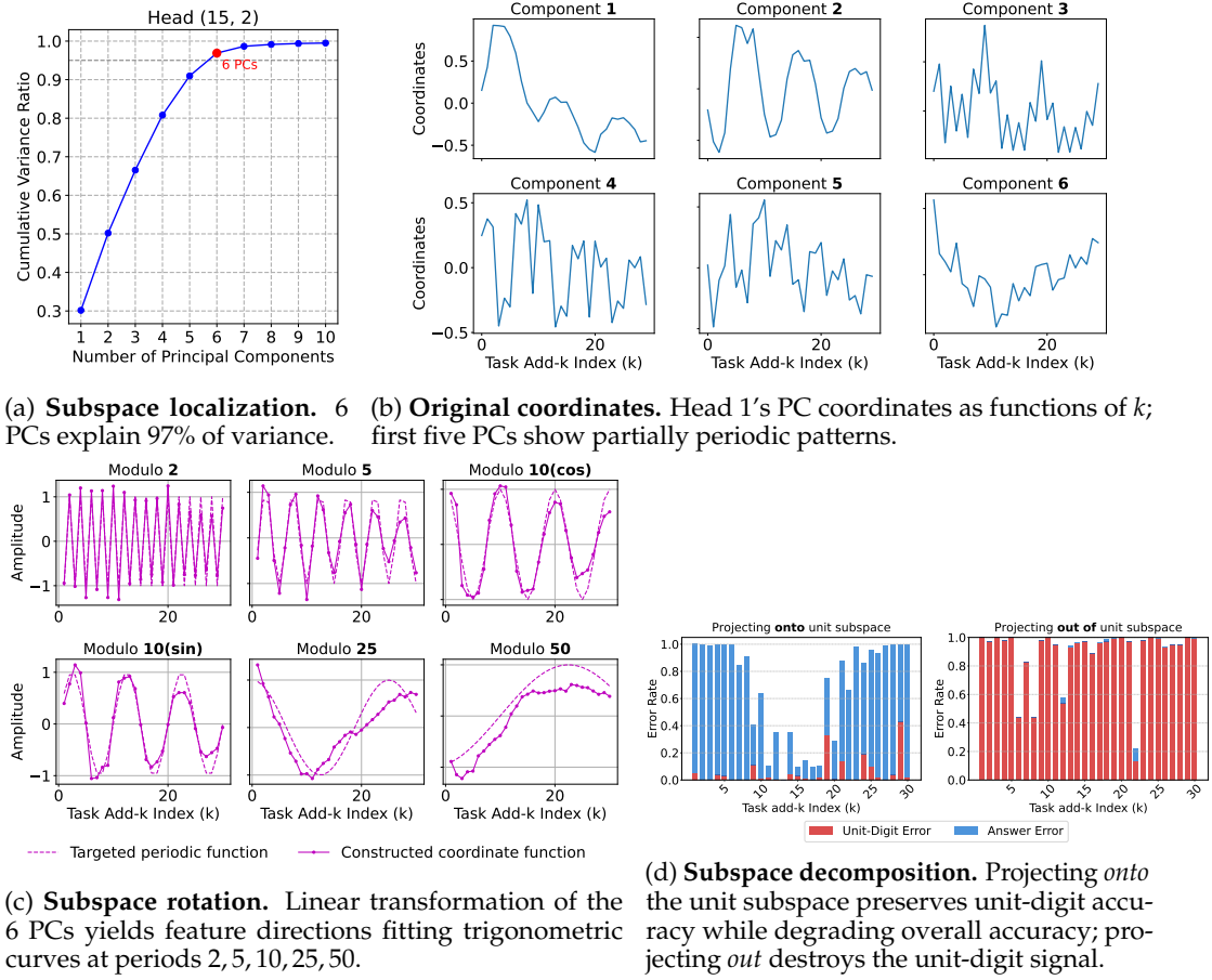
Figure 3: Characterizing the aggregator subspace, illustrated on head 1, (15, 2) (other heads and models in Appendices C–E): (a) PCA localizes task information to a 6-d subspace; (b) PC coordinates show periodic dependence on k ; (c) rotated feature directions encode clean trigonometric patterns; (d) causal steering validates the unit-digit subspace decomposition.
