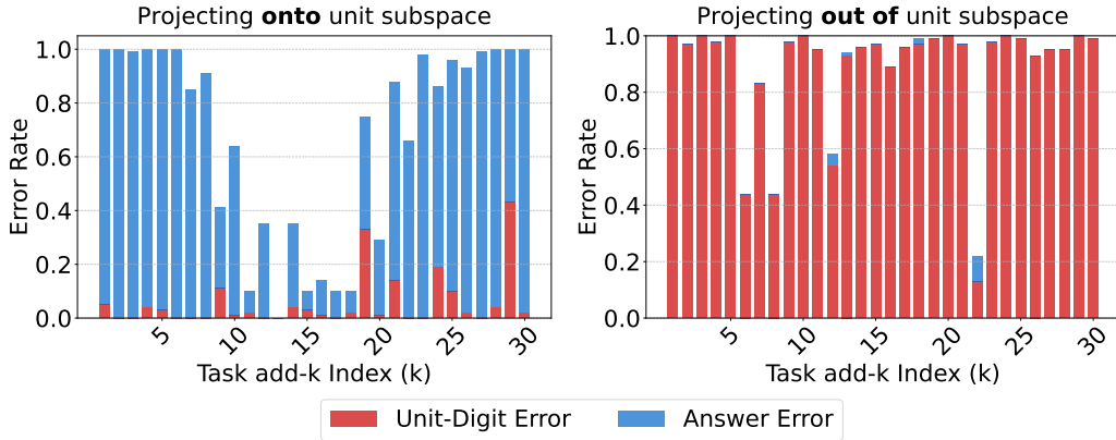
Figure 11: The error rates for the units digit and the final answer across tasks when projecting head 1’s vectors onto (left) and out of (right) the “unit subspace”. Projecting onto the unit subspace yields a low unit-digit error rate even when the final-answer error remains high, while projecting out leads to high unit-digit error rates that almost fully account for final-answer errors. This confirms that the unit subspace encodes the unit-digit signal.
