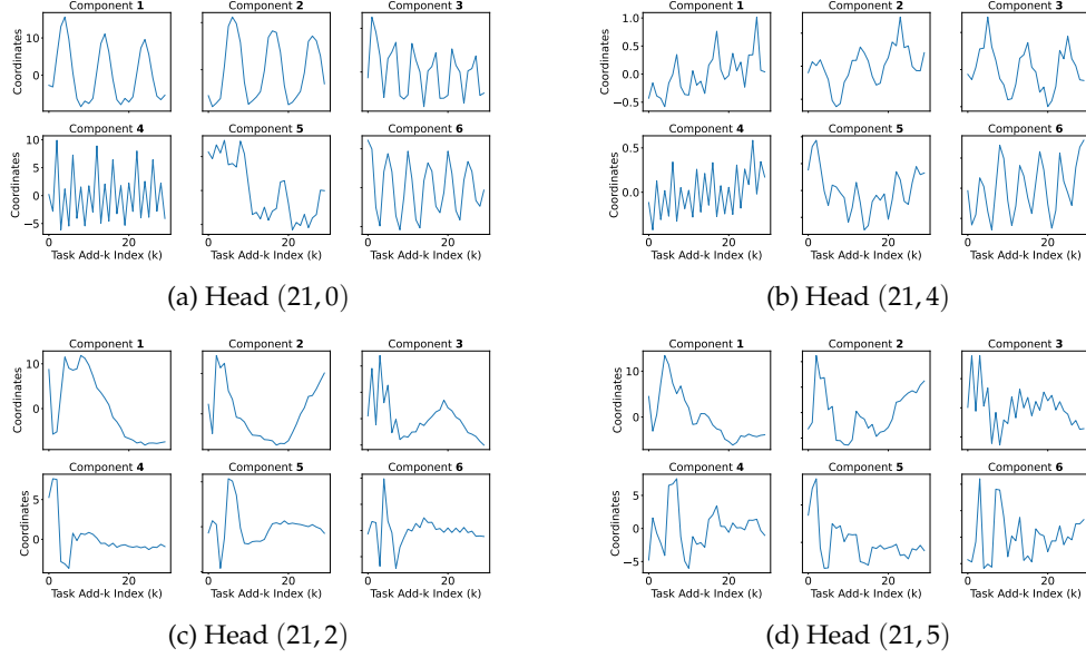
Figure 9: Coordinates of the four Qwen-2.5-7B main heads' vectors (inner products with PCs) for the first six PCs across different add-k tasks. Heads (21,0) and (21,4) reveal periodic patterns, whereas heads (21,2) and (21,5) show discontinuous behaviors across the intervals [1, 10] , [11, 20] , and [21, 30] .
