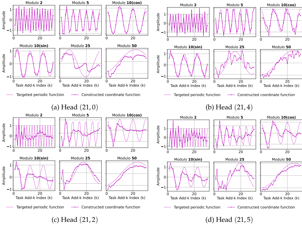
Figure 10: Six trigonometric functions with periods 2, 5, 10, 10, 25, and 50 fitted by the coordinate functions of the four Qwen-2.5-7B main heads. Heads (21,0) and (21,4) fit the periodic functions well, while heads (21,2) and (21,5) fit only the low-frequency directions, consistent with their non-periodic coordinate behaviors.
