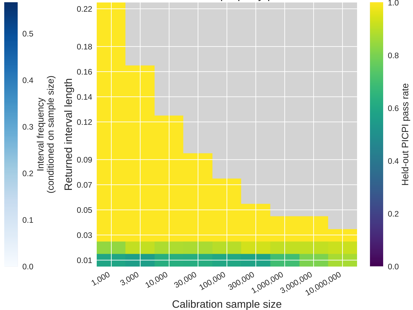
Held-out PICPI property pass rate
