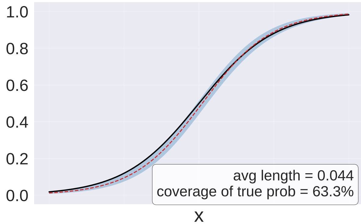
Calibration-based interval
