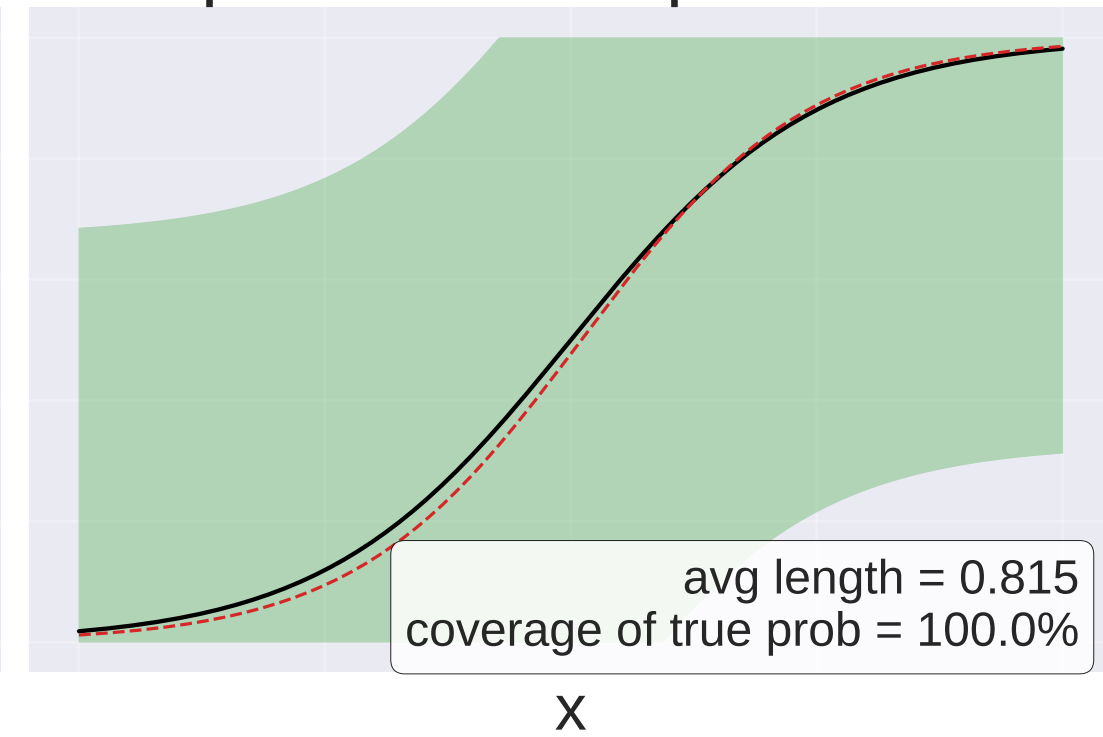
Split conformal prediction
