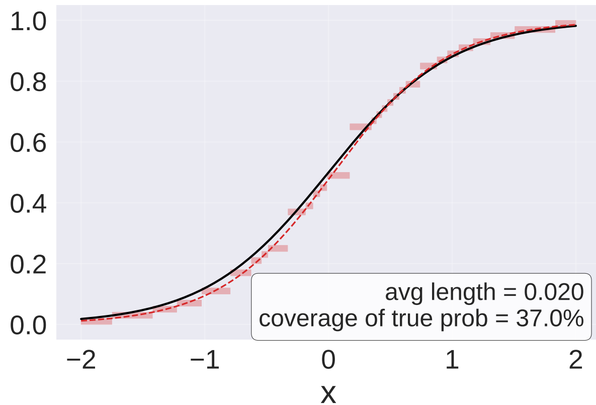
Calibration-based interval
