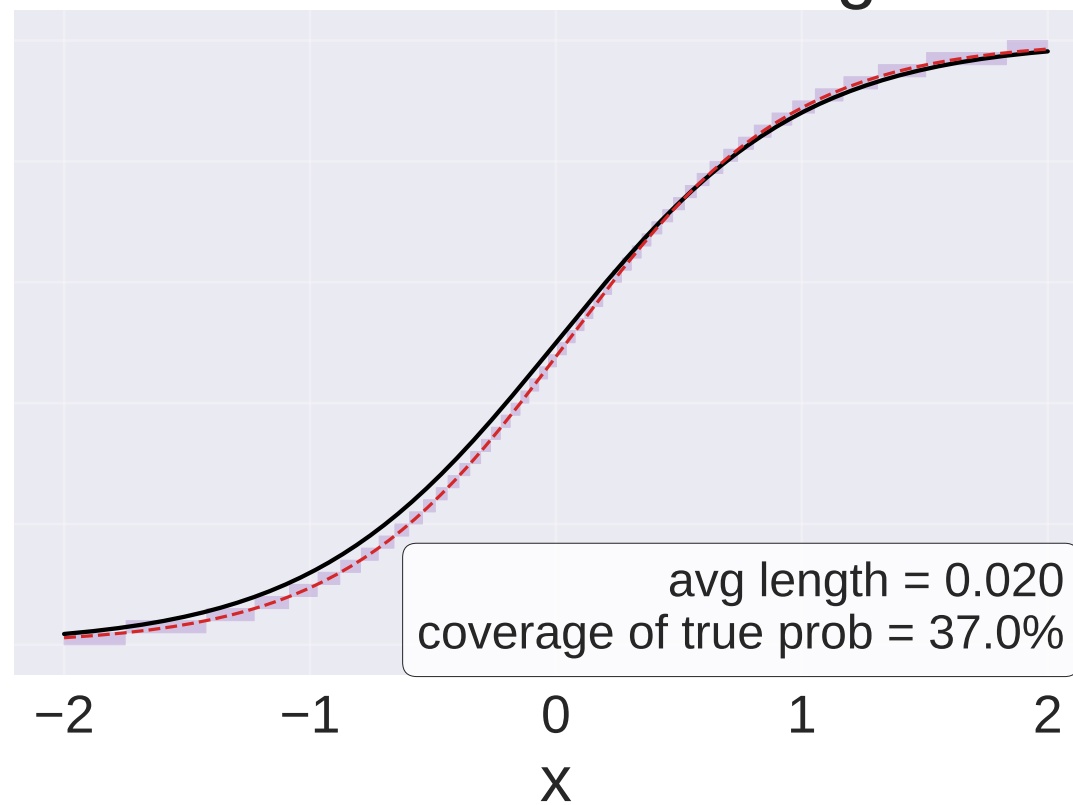
Fixed-width binning
