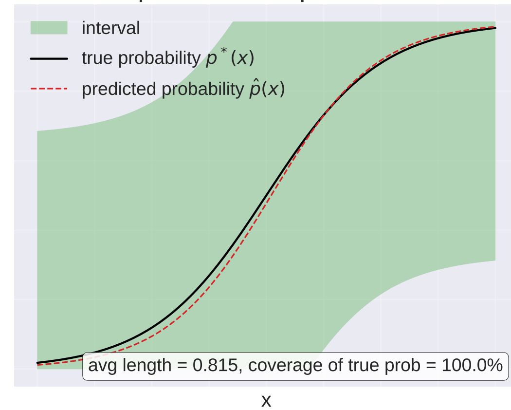
Split conformal prediction
