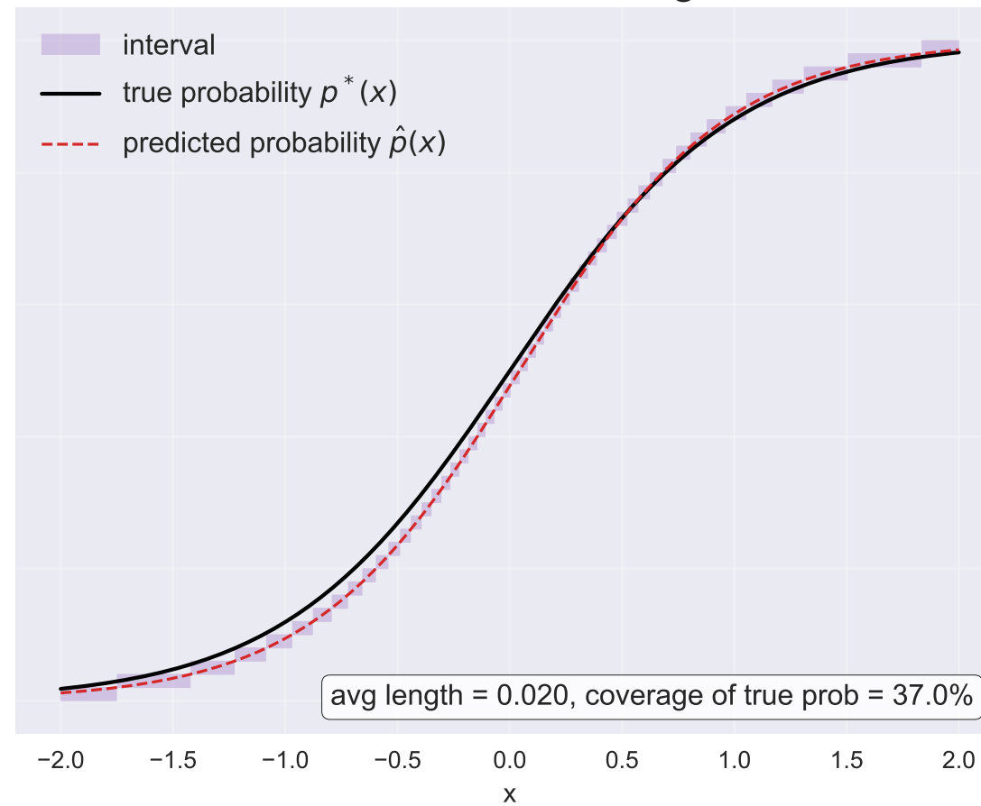
Fixed-width binning
