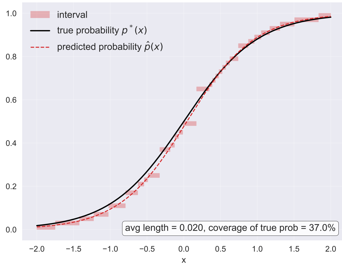
Calibration-based interval
