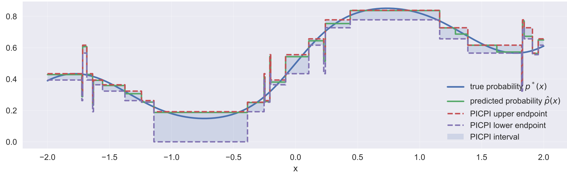
Misspecified point estimator: decision tree
