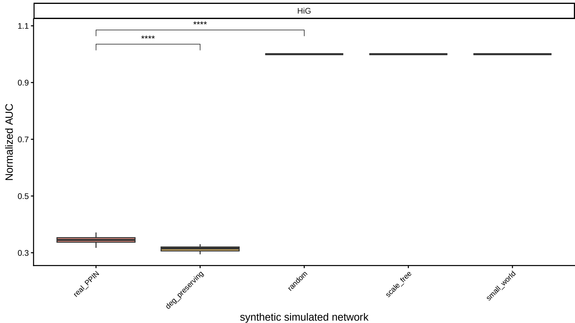
Comparison of normalized AUC across networks within each category
