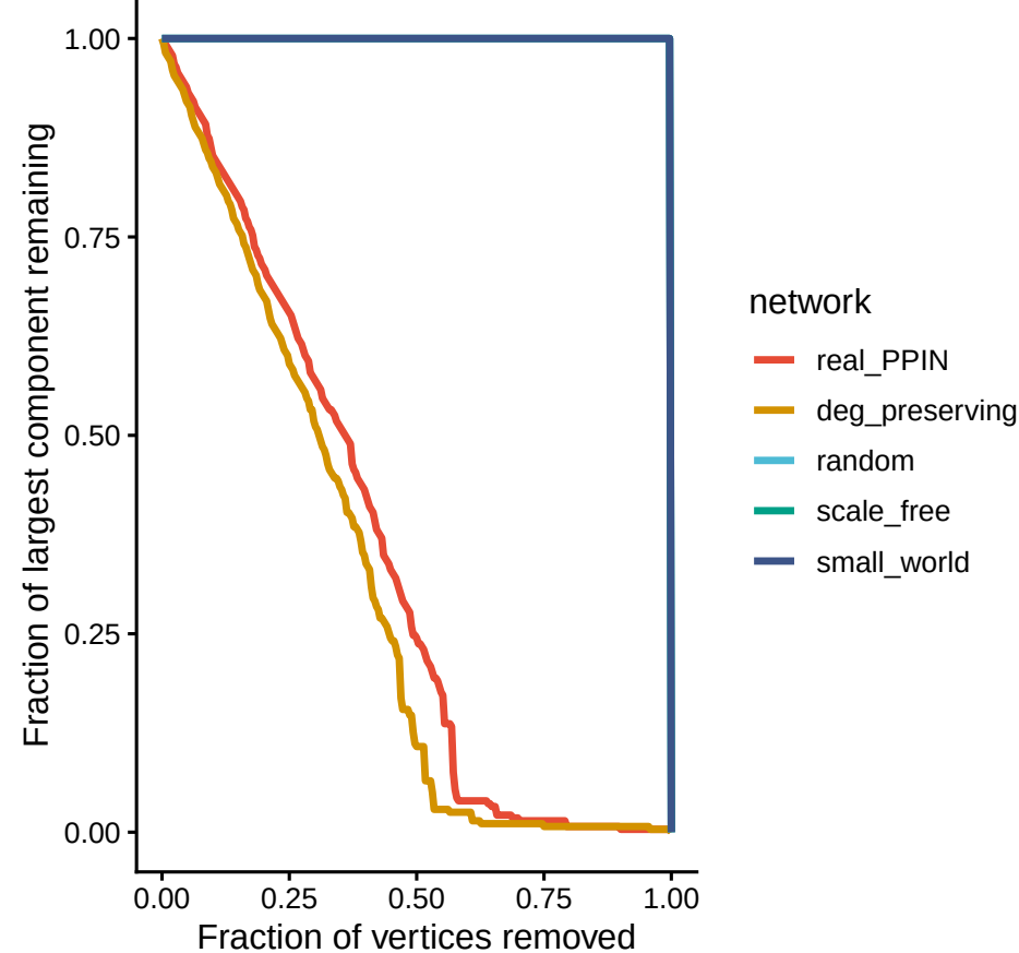
HiG_8 fragmentation under targeted-node attack
