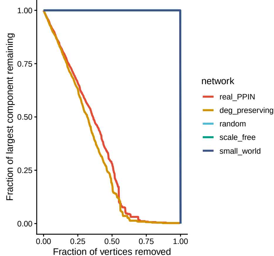
HiG_6 fragmentation under targeted-node attack
