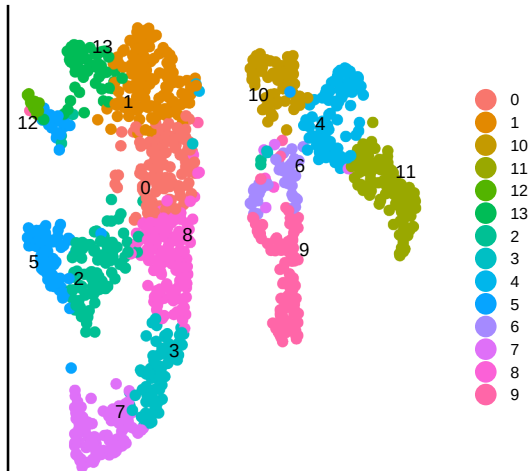
attractor
