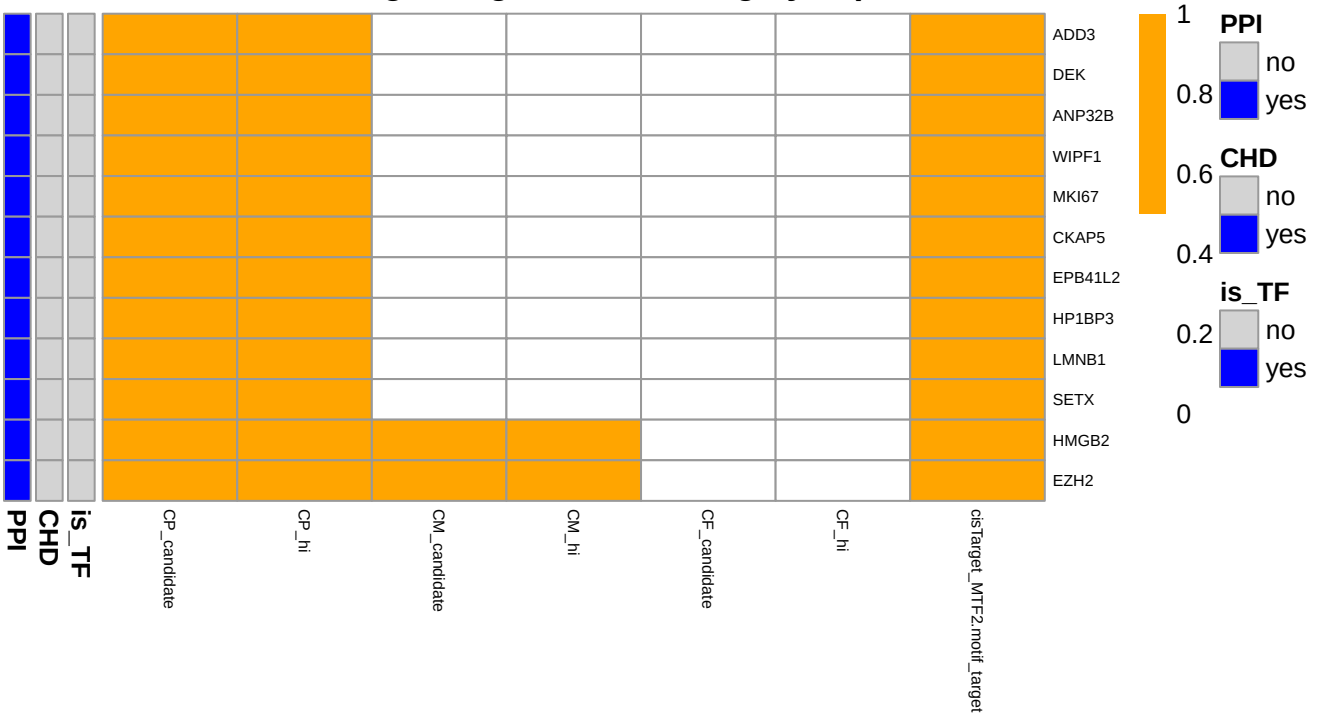
candidate: MTF2 cisTarget targets that are highly expressed in a state
