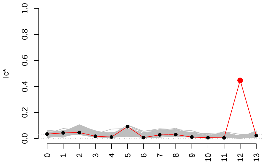
Cluster 12_ 50 genes vs. 100 gene-permutations
