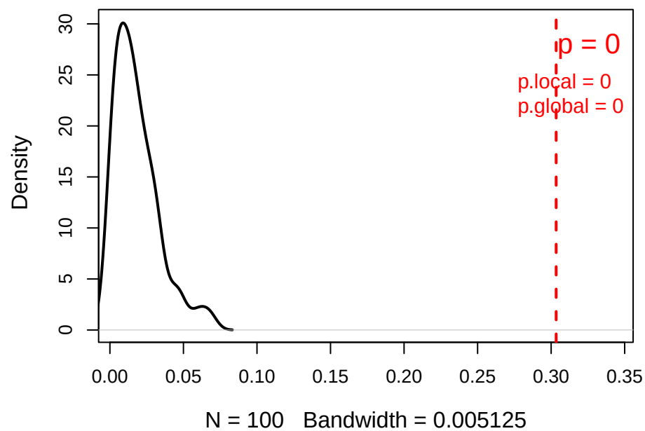
Delta lc^* (cell perm) 89 genes
