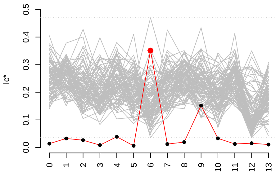
Cluster 6_41 genes vs. 100 cell-permutations
