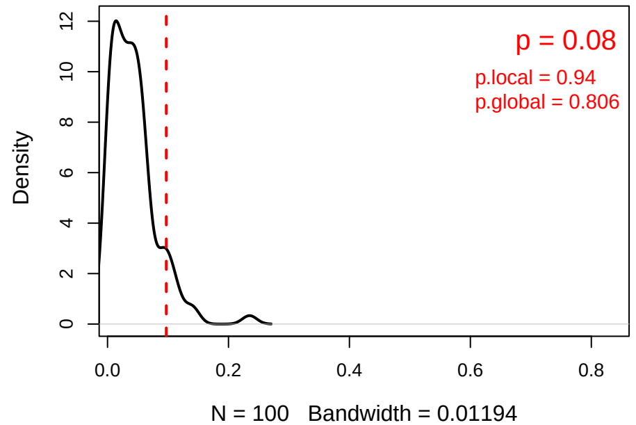
Delta lc^* (cell perm) 101 genes
