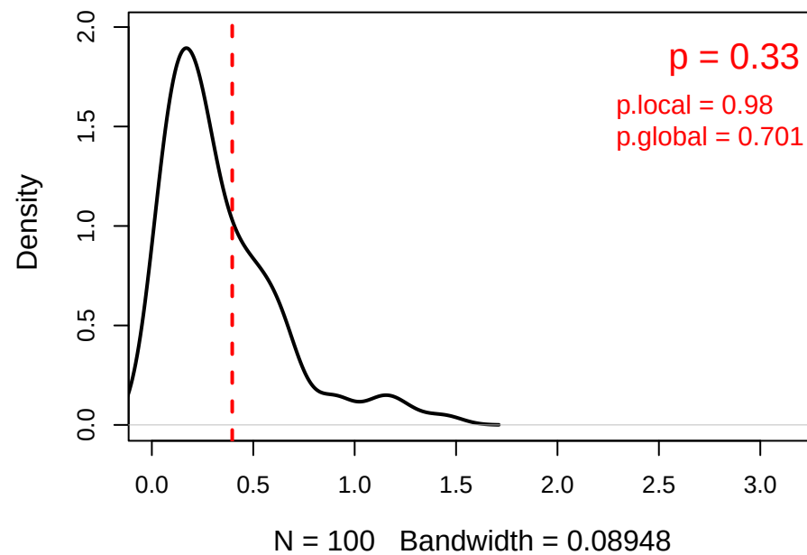
Delta lc^* (cell perm) 31 genes
