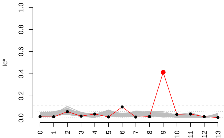
Cluster 9_87 genes vs. 100 gene-permutations
