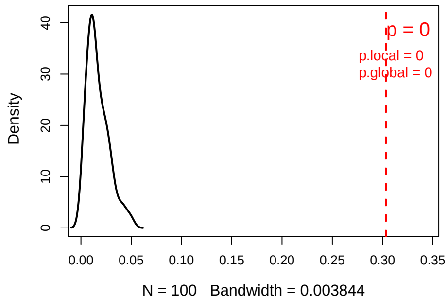
Delta lc^* (gene perm) 89 genes
