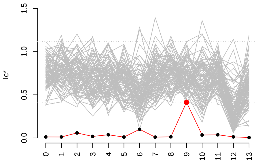
Cluster 9_87 genes vs. 100 cell-permutations
