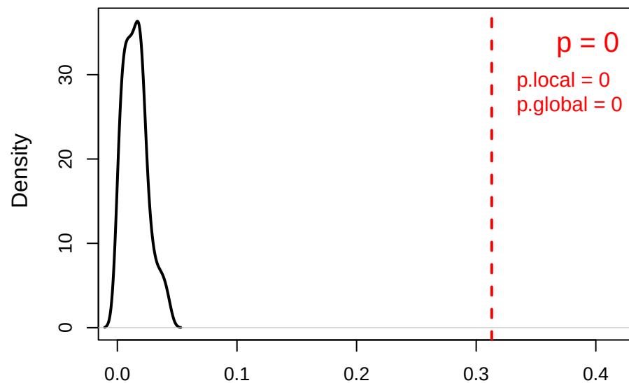
Delta lc^* (gene perm) 87 genes
