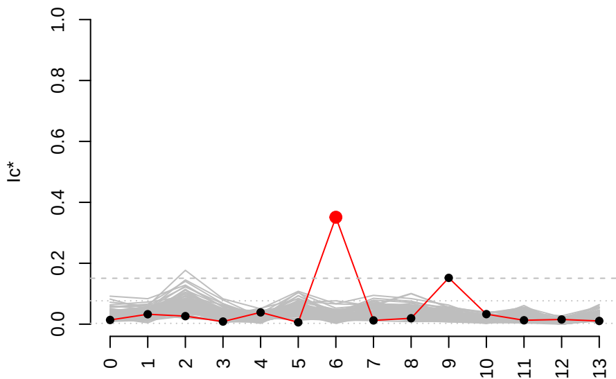
Cluster 6_41 genes vs. 100 gene-permutations
