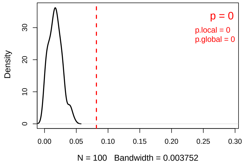
Delta lc^* (gene perm) 86 genes
