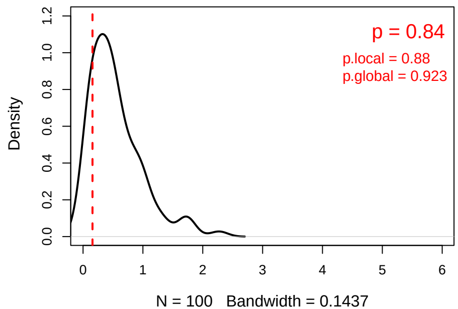
Delta lc^* (cell perm) 76 genes
