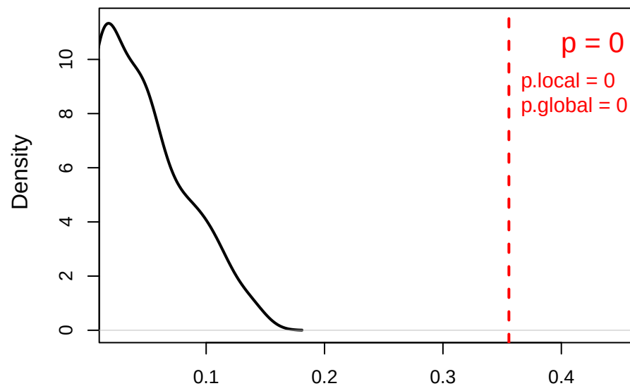
Delta lc^* (cell perm) 50 genes
