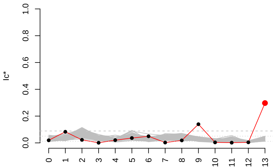
Cluster 13 _ 76 genes vs. 100 gene-permutations
