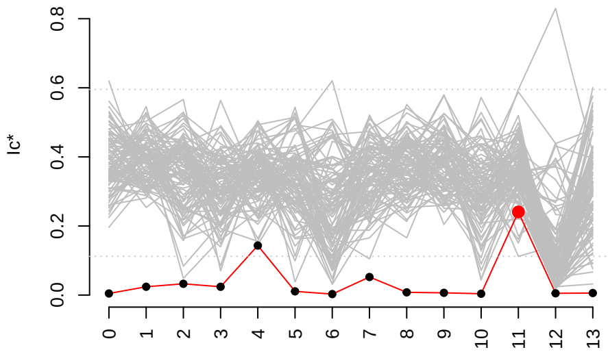
Cluster 11_101 genes vs. 100 cell-permutations
