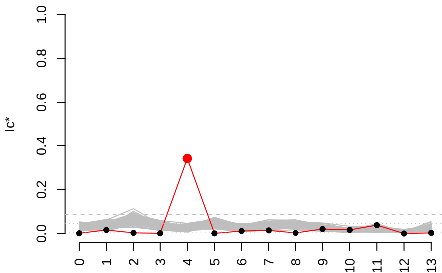
Cluster 4_ 89 genes vs. 100 gene-permutations
