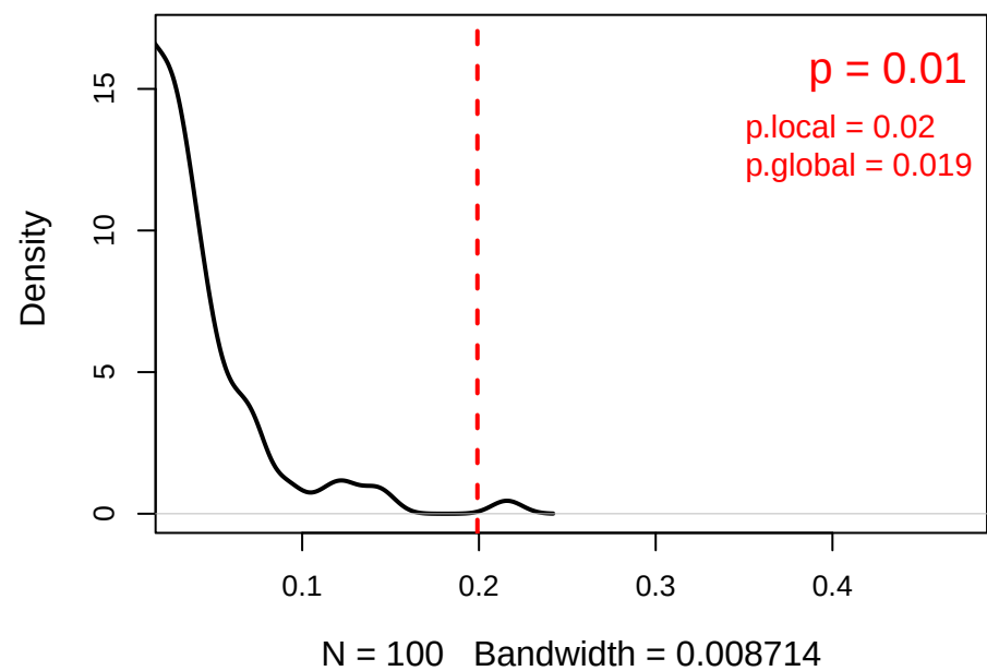
Delta lc^* (cell perm) 41 genes
