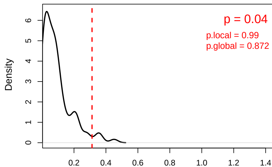
Delta lc^* (cell perm) 87 genes
