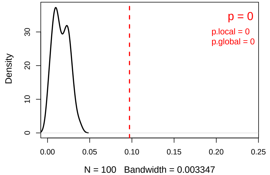
Delta lc^* (gene perm) 101 genes
