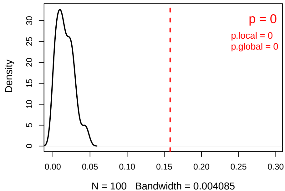
Delta lc^* (gene perm) 76 genes
