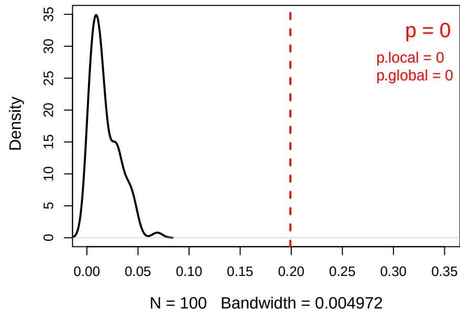
Delta lc^* (gene perm) 41 genes
