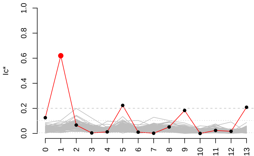
Cluster 1_ 31 genes vs. 100 gene-permutations
