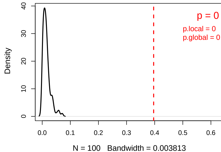
Delta lc^* (gene perm) 31 genes
