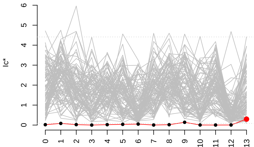
Cluster 13 _ 76 genes vs. 100 cell-permutations
