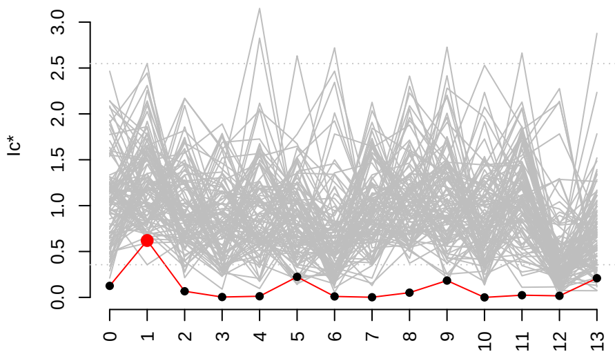
Cluster 1_ 31 genes vs. 100 cell-permutations
