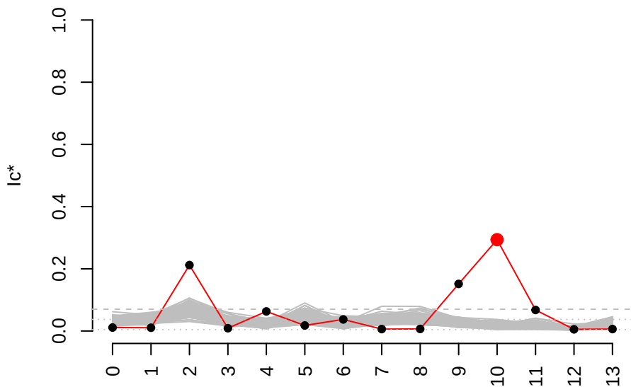
Cluster 10 _ 86 genes vs. 100 gene-permutations
