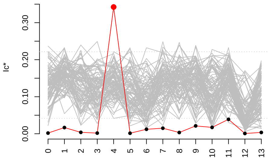
Cluster 4_ 89 genes vs. 100 cell-permutations
