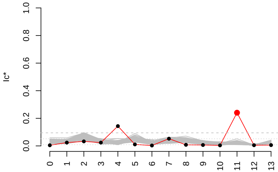
Cluster 11_101 genes vs. 100 gene-permutations
