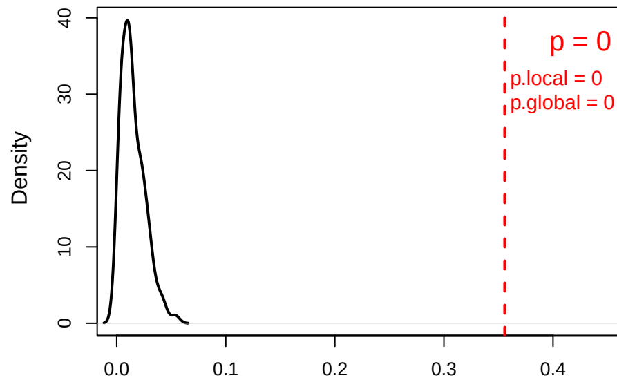
Delta lc^* (gene perm) 50 genes
