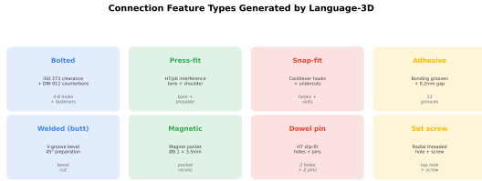
Fig. 2. Eight connection types with real CAD features. Each generates geometry-specific boolean operations (clearance holes, interference bores, snap hooks, etc.).
