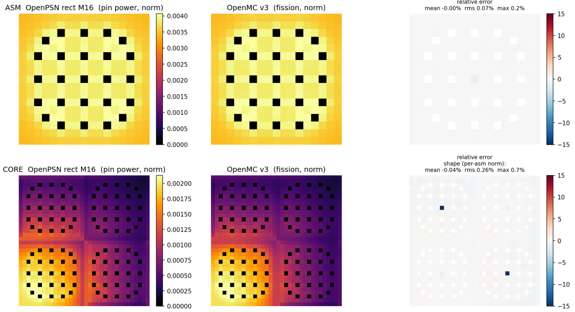
Figure 4: Pin-averaged fission-rate map, rectangular-node OpenPSN ( M=16 , pure XS) vs. OpenMC v3 (explicit geometry, collision estimator). One row per problem — single \text{UO}_2 assembly ( 17 \times 17 pins), then C5G7-2D 1/4 core, fuel region only ( 34 \times 34 pins); columns are OpenPSN (pin power \nu \Sigma_f \phi ), OpenMC (fission count \Sigma_f \phi ), and the relative error, both maps self-normalised per problem (assembly: one normalisation; core: one per 17 \times 17 sub-assembly, which also removes the uniform \nu -weighting offset).
