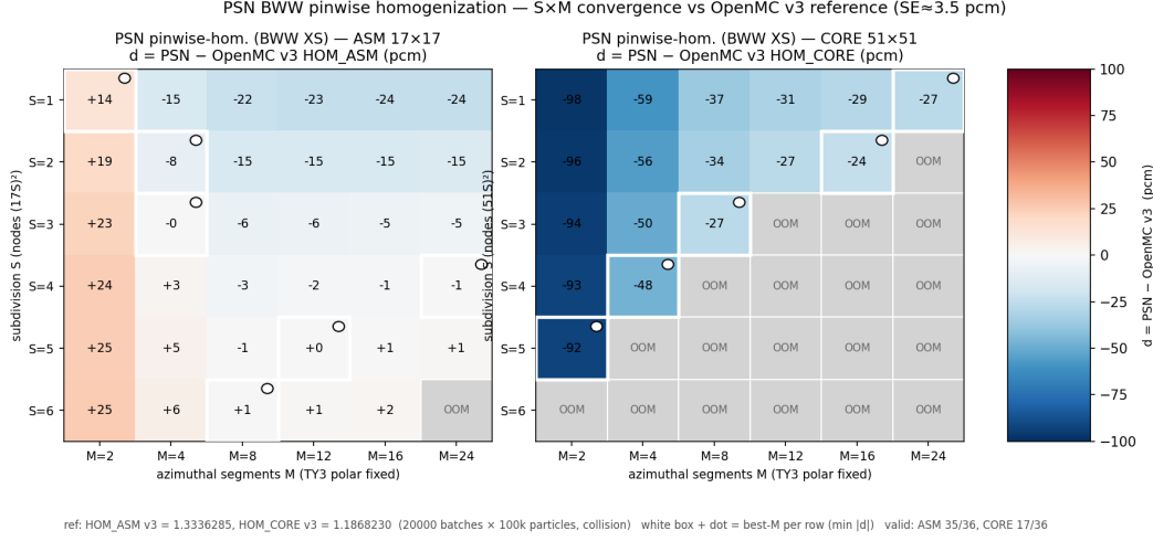
Figure 1: Pinwise-homogenised (BWW) OpenPSN \Delta\kappa_{\text{eff}} in pcm versus the OpenMC v3 homogenised reference, as a function of angular order M (horizontal) and spatial sub-division S (vertical). Left: single UO 2 assembly (ref. 1.3336285, 35 of 36 points computed); right: C5G7-2D 1/4 core (ref. 1.1868230, 17 of 36 points; grey cells exceeded the 64 GB LU fill-in cap). White box/dot marks the minimum- |\Delta| point per S row.
