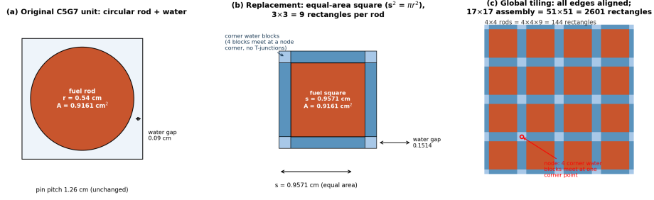
Figure 2: Rectangularisation of the C5G7 pin cell. (a) Original circular rod in its pitch cell (water gap 0.09 cm). (b) Equal-area fuel square ( s = 0.95713 cm, s^2 = \pi r^2 ) with the pin cell split into 3 \times 3 rectangles; the four corner water blocks of neighbouring pins meet at a single node corner, so the tiling has no T-junctions. (c) Global tiling: a 17 \times 17 assembly is 51 \times 51 = 2601 rectangles and the 1/4 core is 153 \times 153 = 23409 .
