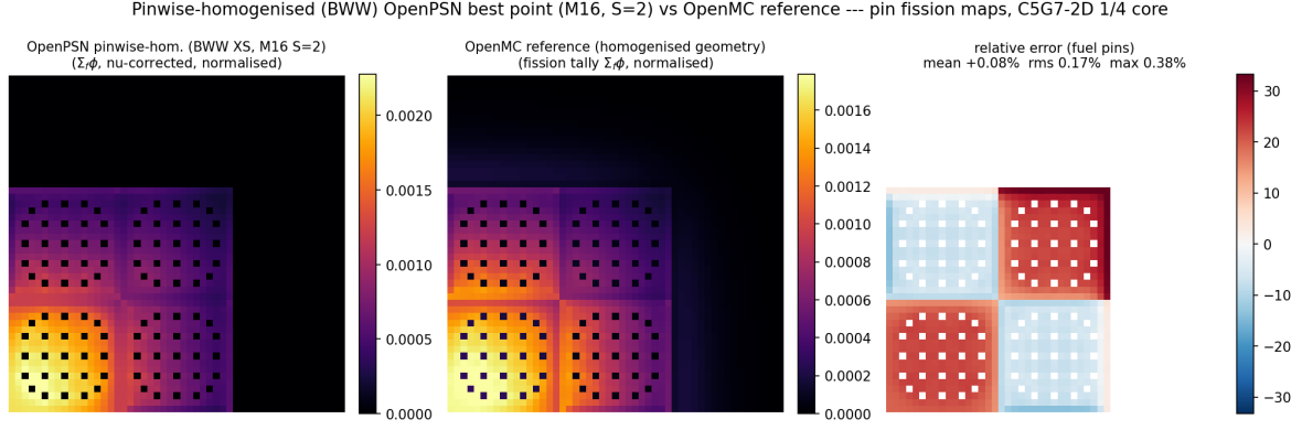
Figure 2: Pin-averaged fission maps \Sigma_f \phi at the best pinwise-homogenised core point (M16, S=2) vs. the OpenMC homogenised-geometry reference on the same BWW XS, C5G7-2D 1/4 core (fuel region, 34 \times 34 pins). Left: OpenPSN ( \nu -corrected); centre: OpenMC reference (7-group, collision); right: relative error (fuel pins only, both maps normalised to unit sum).
