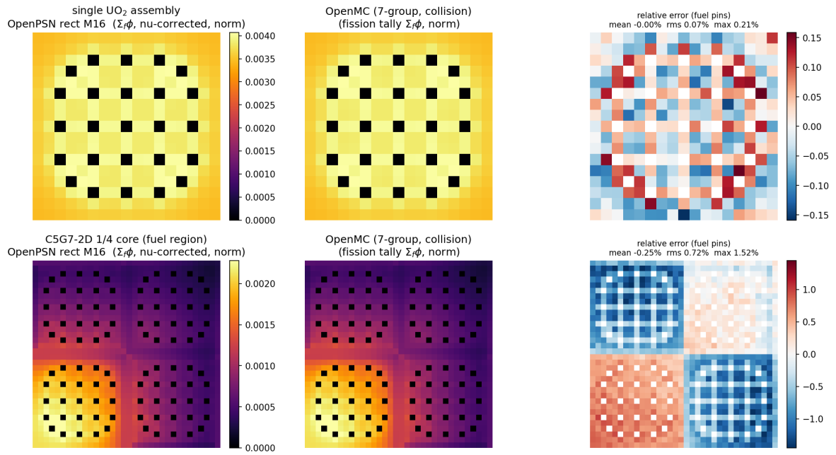
Figure 4: Pin-averaged fission maps \Sigma_f \phi , rectangular-node OpenPSN ( M=16 , un-homogenised material XS, \nu -corrected) vs. OpenMC (explicit geometry, 7-group collision estimator). One row per problem — single UO 2 assembly (17×17 pins), then C5G7-2D 1/4 core, fuel region only (34×34 pins); columns are OpenPSN, OpenMC, and the pin-by-pin relative error (fuel pins only), both maps normalised to unit sum.
