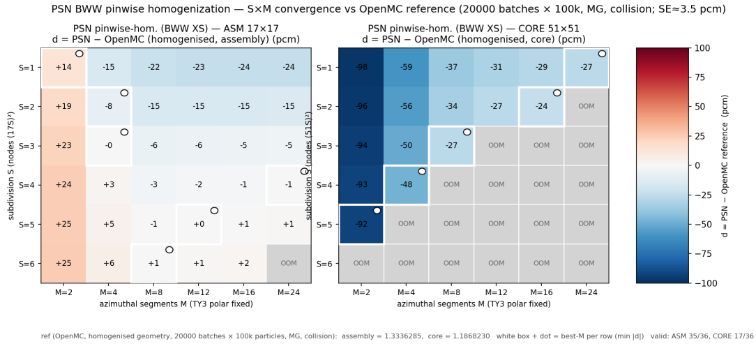
Figure 1: Pinwise-homogenised (BWW) OpenPSN \Delta\kappa_{\text{eff}} in pcm versus the OpenMC homogenised reference, as a function of angular order M (horizontal) and spatial sub-division S (vertical). Left: single UO 2 assembly (ref. 1.3336285, 35 of 36 points computed); right: C5G7-2D 1/4 core (ref. 1.1868230, 17 of 36 points; grey cells exceeded the 64 GB LU fill-in cap). White box/dot marks the minimum- |\Delta| point per S row.
