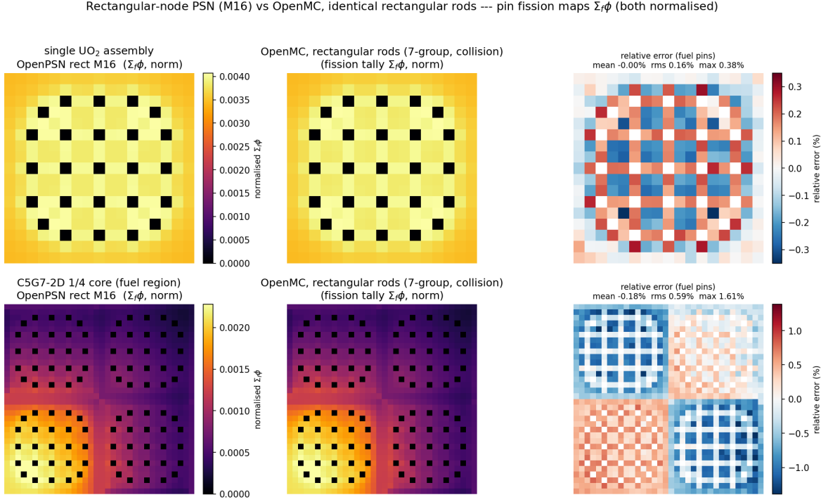
Figure 5: Pin-averaged fission maps \Sigma_f \phi , rectangular-node OpenPSN ( M=16 ) vs. OpenMC on the identical rectangular-rod geometry (equal-area square fuel block per pin cell, 7-group collision estimator). One row per problem — single \text{UO}_2 assembly ( 17 \times 17 pins), then C5G7-2D 1/4 core, fuel region only ( 34 \times 34 pins); columns are OpenPSN, OpenMC, and the pin-by-pin relative error (fuel pins only), both maps normalised to unit sum.
