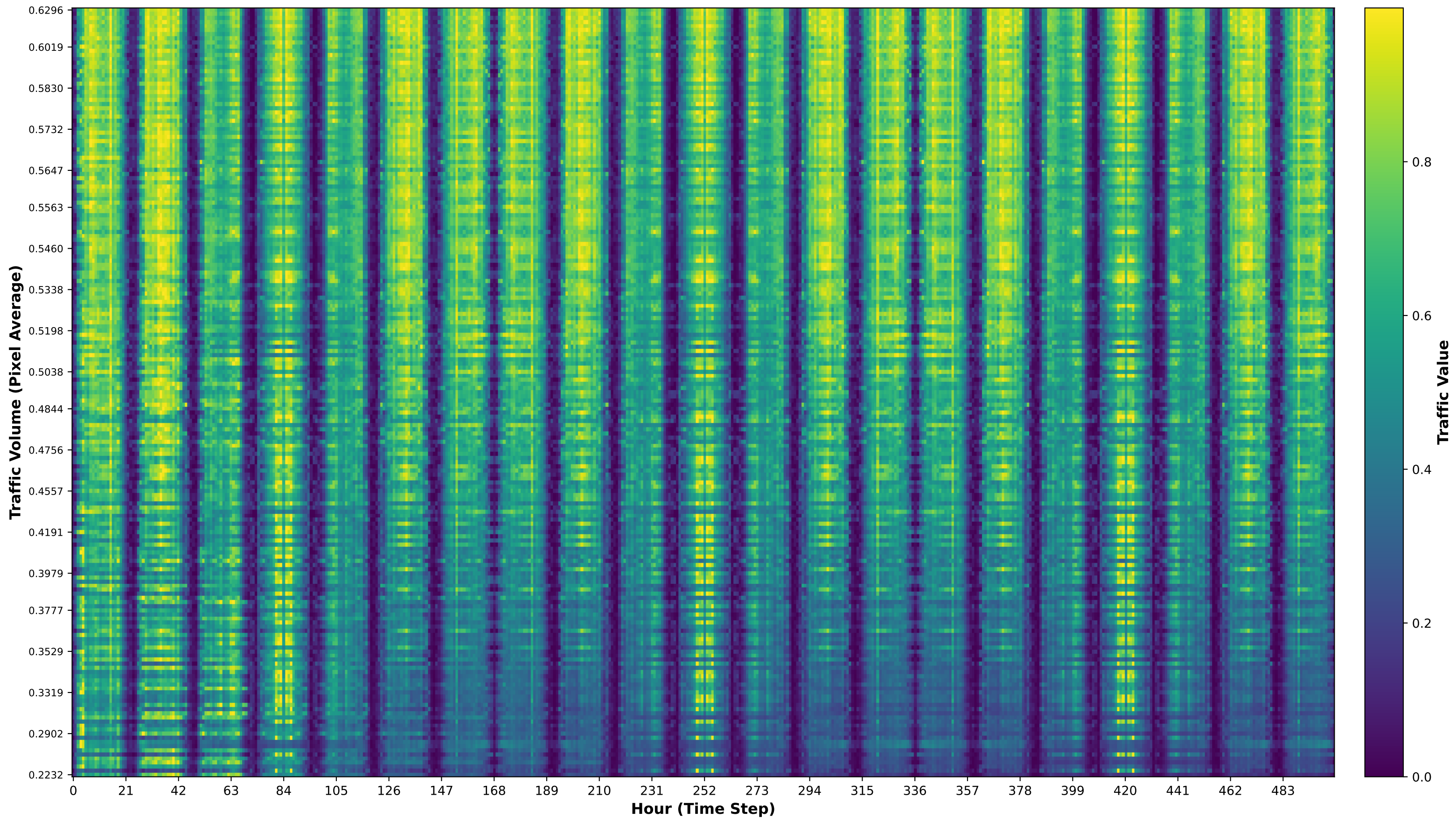
Aachen - Traffic Time Series per Pixel (Sorted by Traffic Volume) (X-axis: Hour, Y-axis: Traffic Volume, Color: Traffic)
