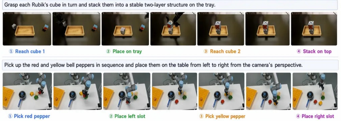
Figure 5: Fine-grained language grounding. (a) Contrastive: each pair of columns shares an identical initial frame (colored border); only the highlighted keyword differs between the two instructions. Pair 1: target object identity. Pair 2: destination. Pair 3: action type. In every case the generated motion is precisely grounded to the discriminating keyword. (b) Complex: two examples requiring multi-step execution or abstract goal inference. Colored labels mark key action milestones within each generated sequence.
