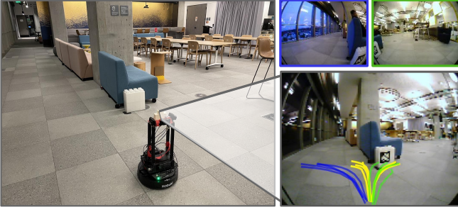
Fig. 3: Visualizing the task-agnostic (yellow) and goal-directed pathways for two goal images (green, blue) learned by NoMaD. NoMaD predicts a bimodal distribution of collision-free actions in the absence of a goal, and snaps to a narrower distribution after conditioning on two different goal images.
