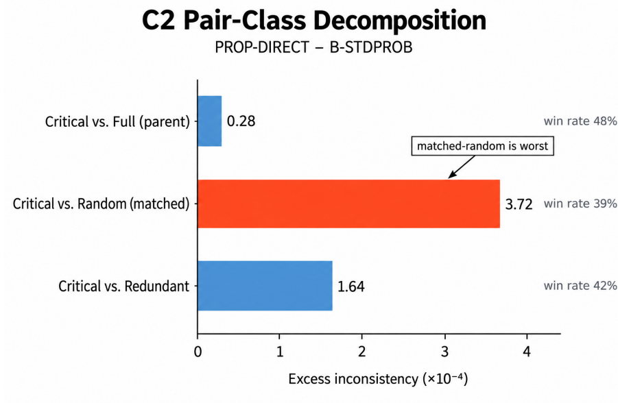
Figure 3: Information-loss pair-class decomposition. Excess inconsistency relative to B-STDPB is small for critical-versus-full comparisons but substantially larger for the matched-random class. The associated win rates show the same ordering, isolating the sensor-importance blindness pattern.
