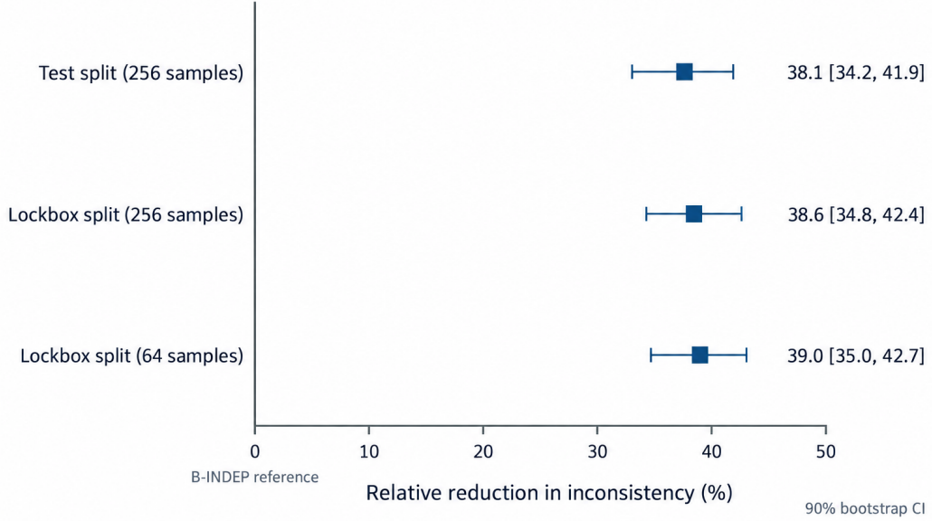
Figure 2: Primary consistency result. PROP-DIRECT reduces cross-view posterior inconsistency relative to B-INDEP by approximately 38% on both the test and lockbox splits. Squares show point estimates and horizontal bars show 90% bootstrap confidence intervals; the reduced 64-sample budget produces the same conclusion.
