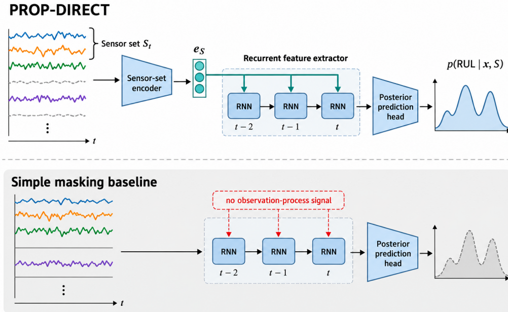
Figure 1: Observation-process conditioning in PROP-DIRECT. The model encodes the available sensor set as e_S and injects that representation into each recurrent step before predicting the RUL posterior. The lower strip shows the masking baseline, which replaces missing values but provides no explicit observation-process signal.
