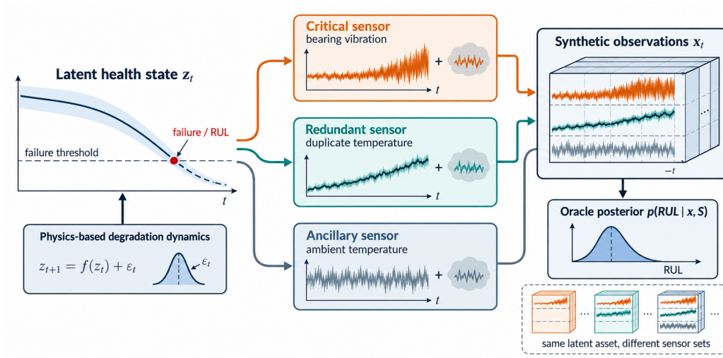
Figure 4: Synthetic degradation-data generator. A latent health state evolves under physics-based dynamics and crosses a failure threshold at the true RUL. Noisy observation channels produce critical, redundant, and ancillary sensors, while different sensor subsets of the same latent asset support exact oracle-posterior computation.
