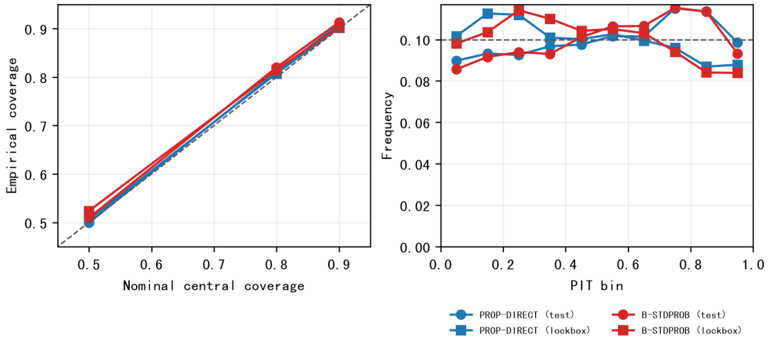
Figure 8: Posterior calibration diagnostics. Left: empirical central coverage at nominal 50%, 80%, and 90% levels, averaged over the three joint coordinates. Right: PIT histograms with the uniform reference shown by the dashed line. Circles and squares denote test and lockbox splits; the plots are descriptive checks rather than additional decision gates.
