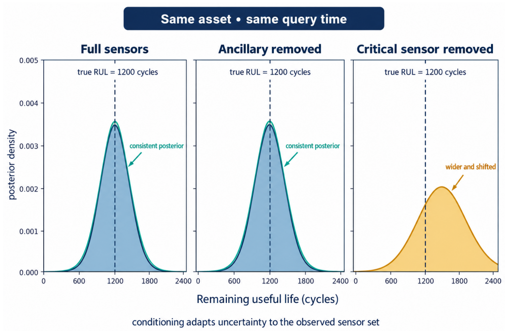
Figure 6: Illustrative prediction under changing sensor sets. For the same asset and query time, full sensors and ancillary-sensor removal produce closely overlapping posteriors, while critical-sensor removal yields a wider and shifted distribution. The example gives an operational interpretation of cross-view consistency and its importance-dependent boundary.
