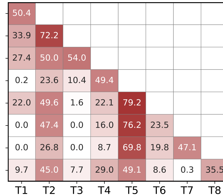
(c) LoRA
