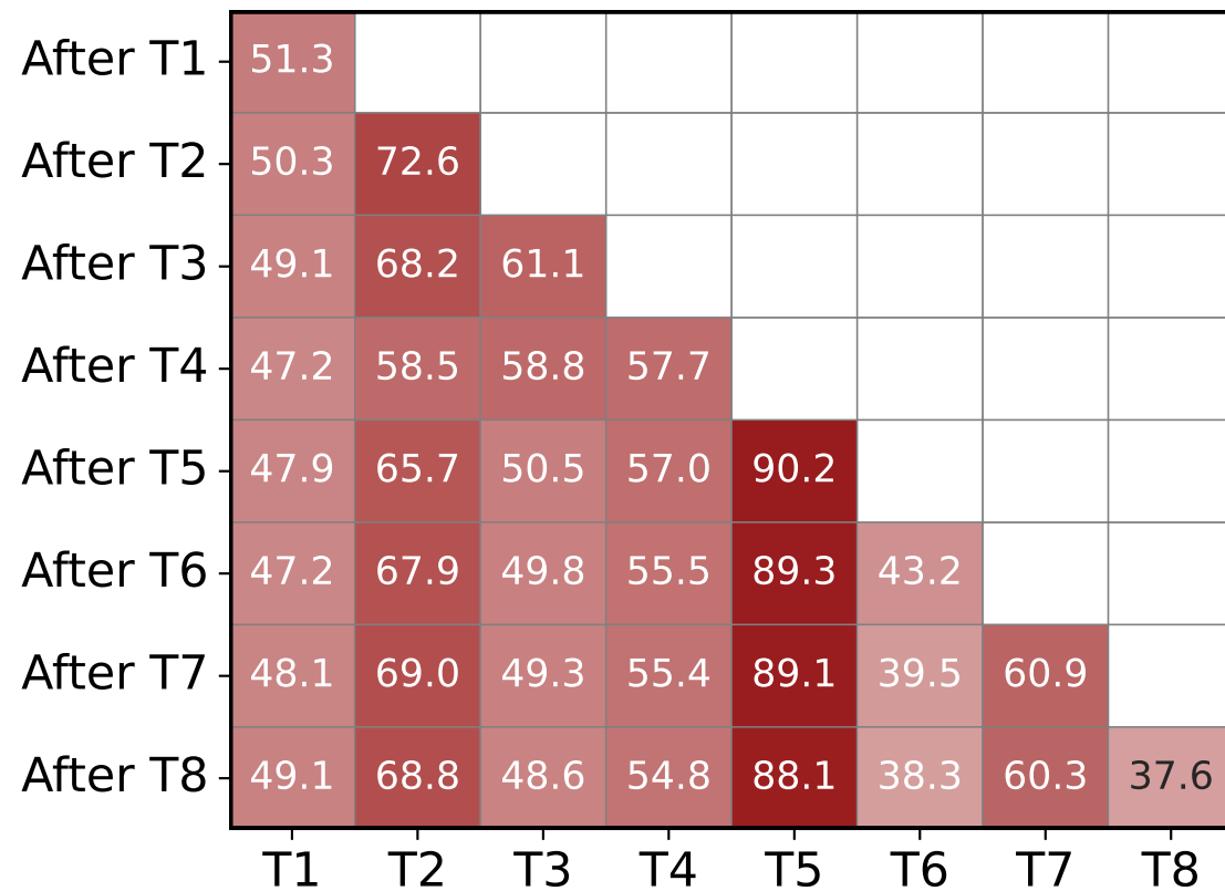
(a) GoD-MOE
