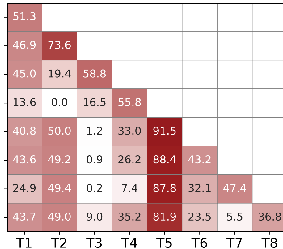
(b) MOE-LoRA
