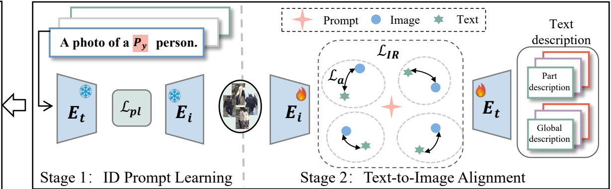
Intra-ID Cross-modal Regularizing (IntraCR)
