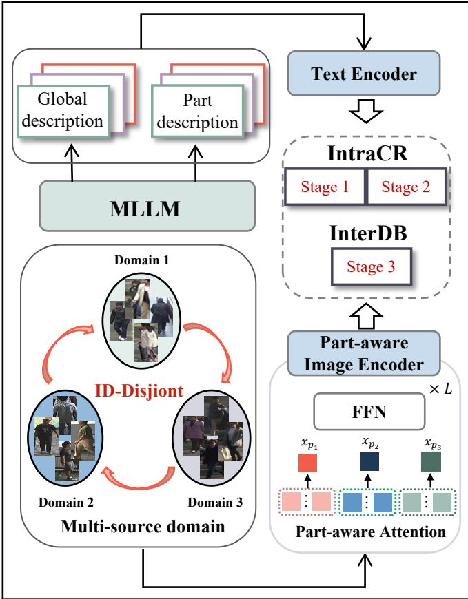
Part-aware CLIP
