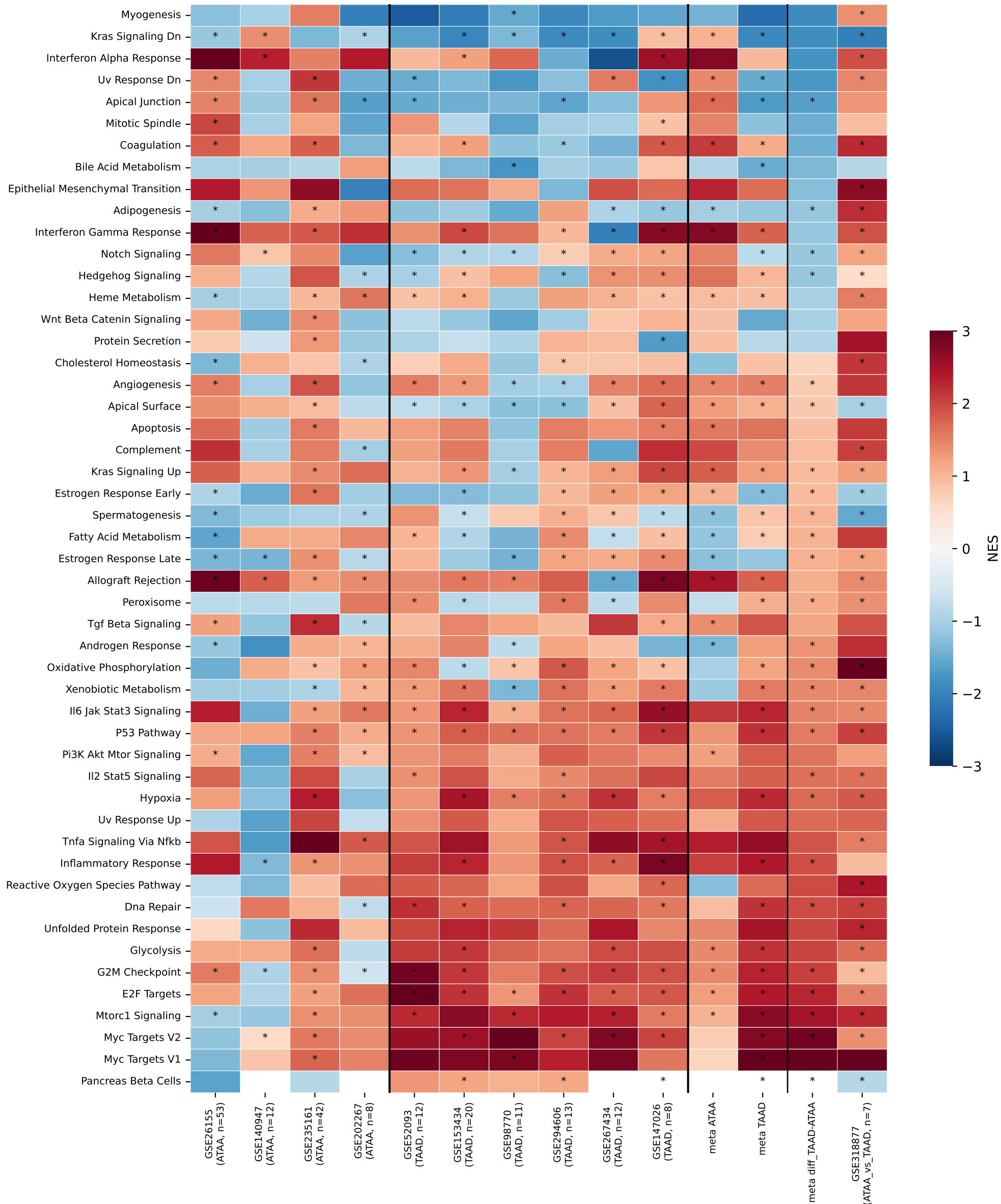
Hallmark GSEA: ATAA cohorts | TAAD cohorts | meta-rankings | direct TAAD-vs-ATAA (GSE318877) (* FDR<0.05)
