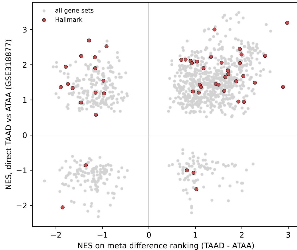
Pathway-level validation in the direct-contrast cohort \rho=0.42 (all), 0.22 (Hallmark)
