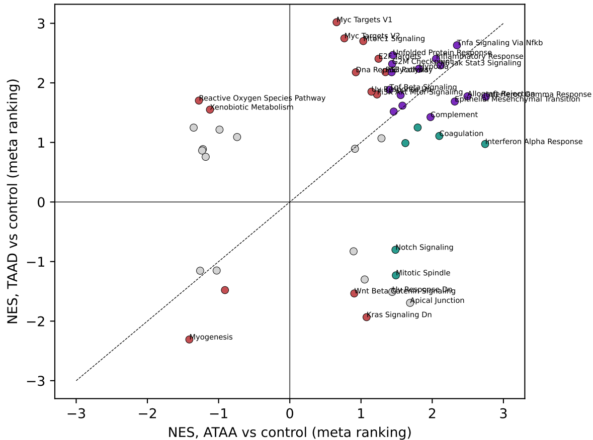
Hallmark pathways: disease-level GSEA
