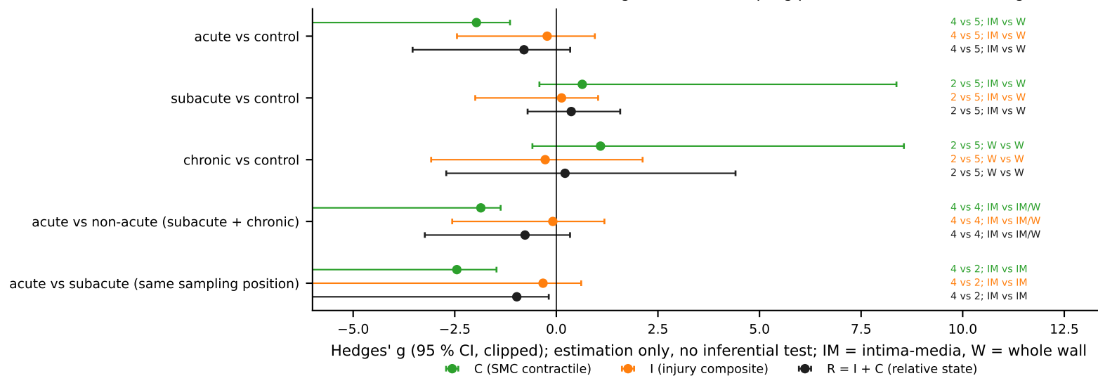
d GSE222318 contractile SMC: stage contrasts (sampling position confounded with stage)
