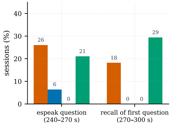
(b) synthetic-voice probes
