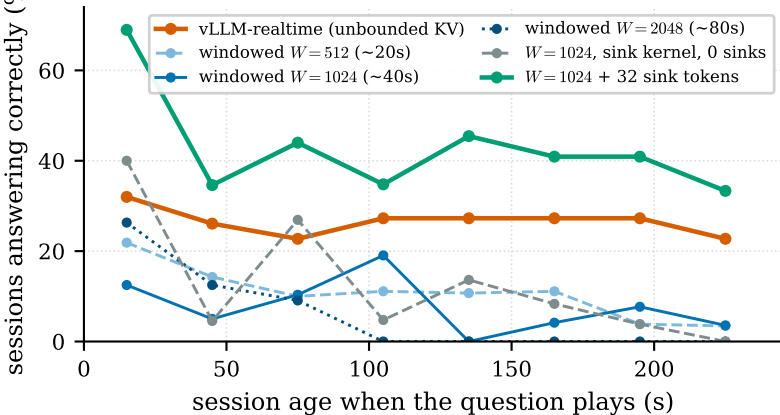
(a) correctness vs session age (rotating questions)
