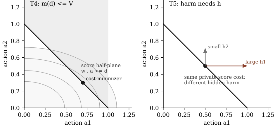
Figure 2: T4 locates the private cost-minimizing action for a score deficit. T5 then requires hidden harm exchange rates before that action can be interpreted as welfare movement.
