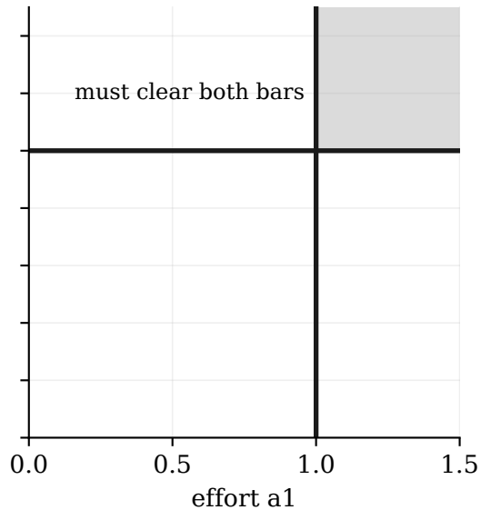
B. conjunctive: a1 \geq t and a2 \geq t
