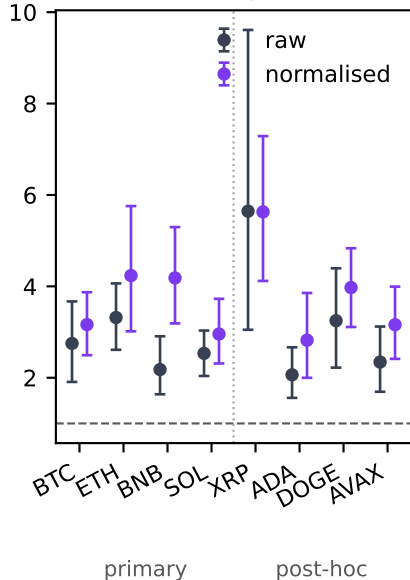
(a) total amplification
