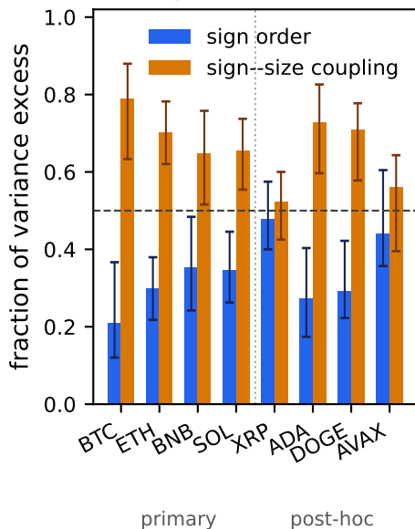
(b) signed base volume
