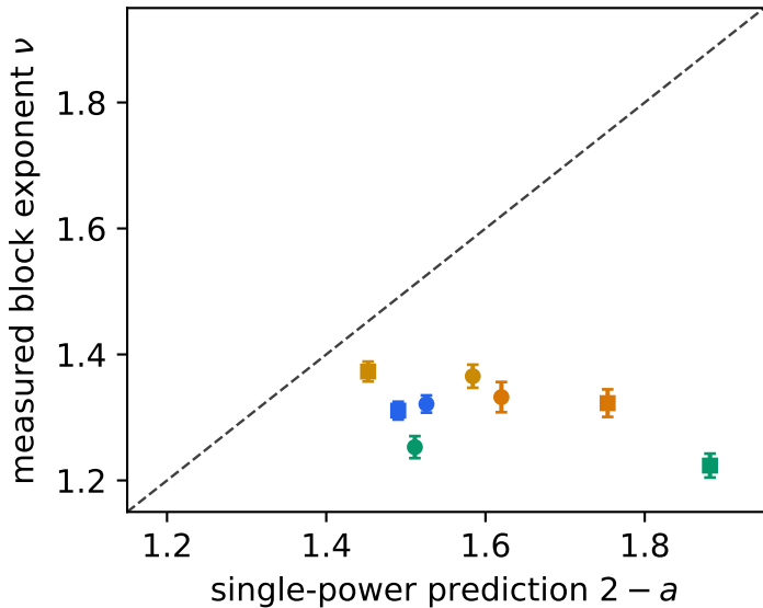
(a) one power fails in all eight series
