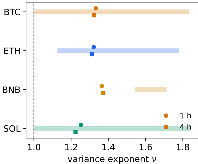
(b) two-regime consistency bands
