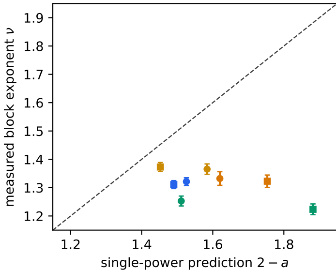
(a) one power fails in all eight series
