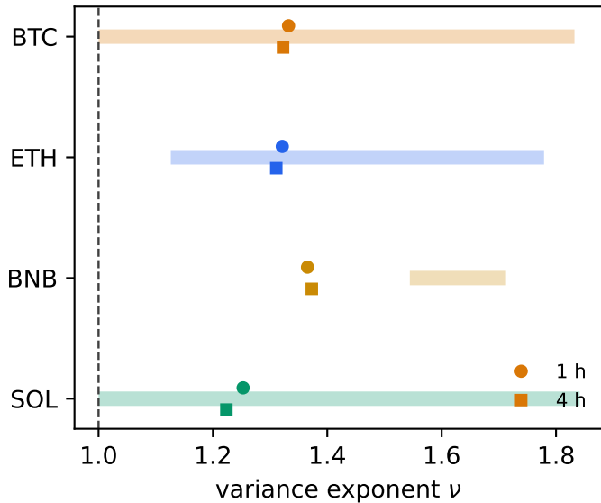
(b) two-regime consistency bands
