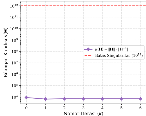
Stabilitas Kurvatur Matriks Hessian
