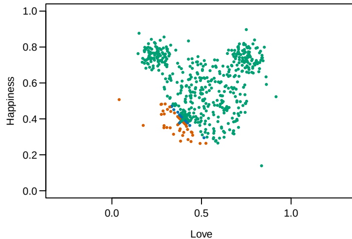
5. R's Lloyd function
