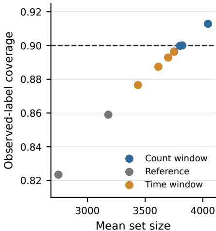
(b) Window ablation at 30% deletion
