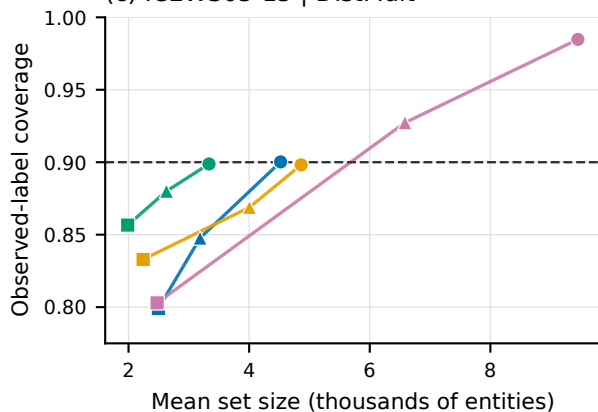
(c) ICEWS05-15 | DistMult
