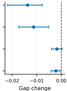
(c) Multi-answer gap
