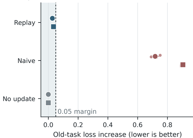
b Retaining the old task
