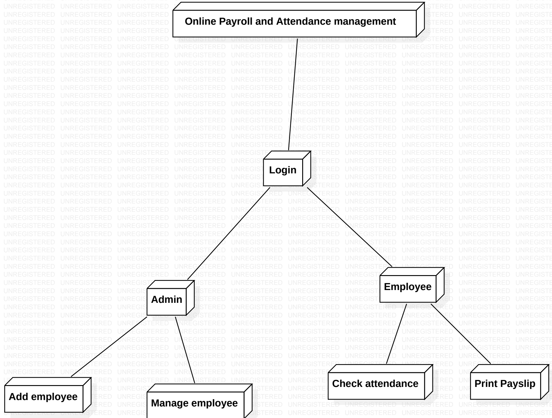
Model1::DeploymentDiagram1
