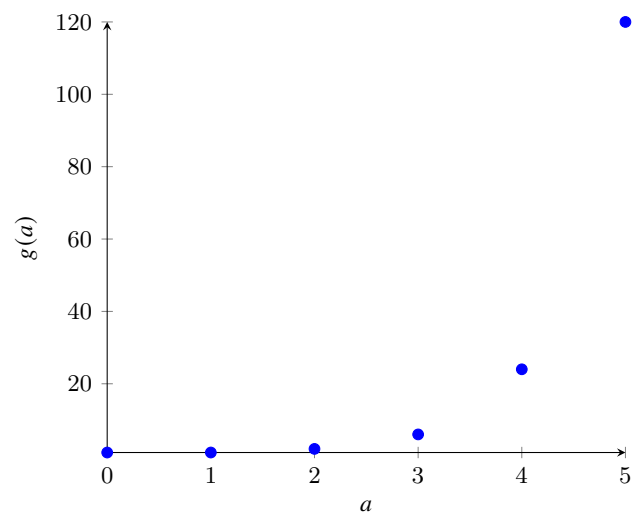
Figure 1.5 Graph of g(a) .
