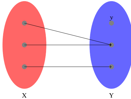
Fig. 1.8 Illustration of non-surjective function with domain X and range Y .
