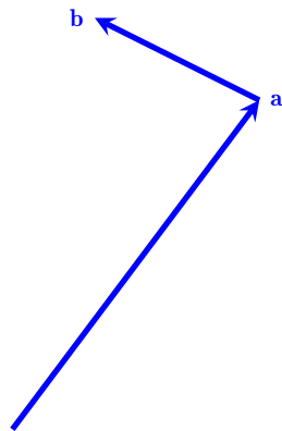
Fig. 2.5 Visualization of “head to tail” addition of a and b .
