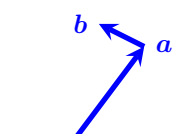
Figure 2.5 Visualisation of “head to tail” addition of \mathbf{a} and \mathbf{b} .
