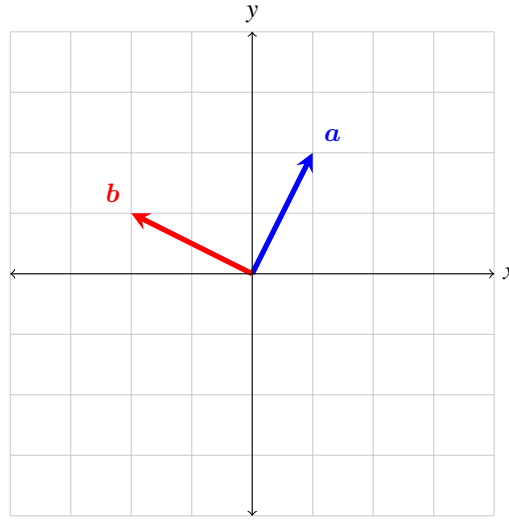
Figure 2.1 Figure of vectors a and b .
