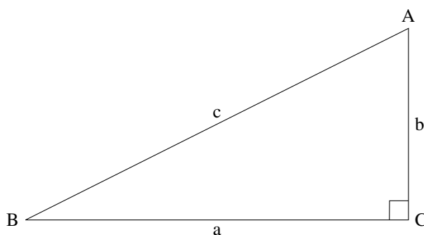
Figure 1.7 Figure of right triangle ABC.
