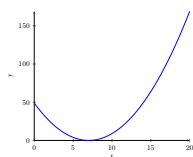
Figure 1.11: Plot of (x - 7)^2 .
