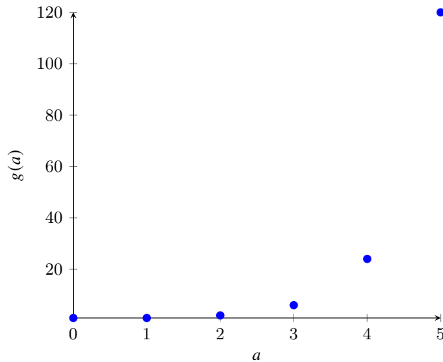
Figure 1.5 Graph of g(a) .
