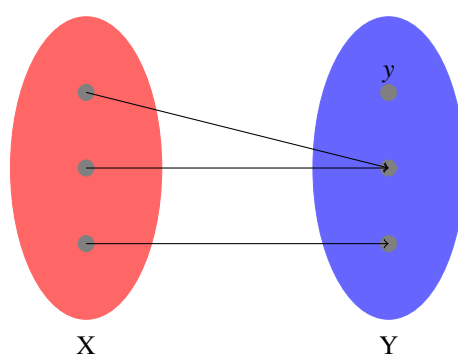
Figure 1.10 Illustration of non-surjective function with domain X and range Y .
