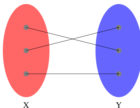
Figure 1.8 Illustration of an injective function with domain X and range Y .
