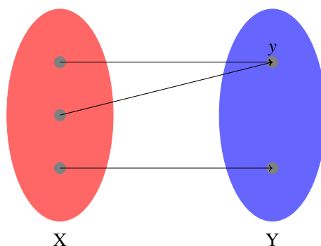
Figure 1.9 Illustration of a non-injective function with domain X and range Y .
