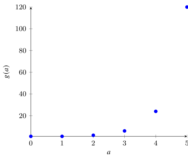
Figure 1.4 Graph of g(a) .
