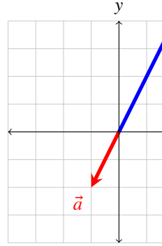
Figure 2.7: Two vectors, one is scaled by -0.5.
