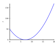
Figure 1.9 Plot of (x - 7)^2 .
