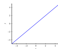
Figure 1.1 Graph of y = x .
