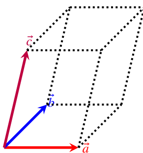
Figure 2.19 Figure of triple vector multiplication.
