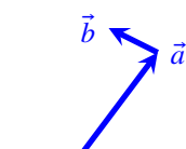
Figure 2.5 Visualisation of “head to tail” addition of \vec{a} and \vec{b} .
