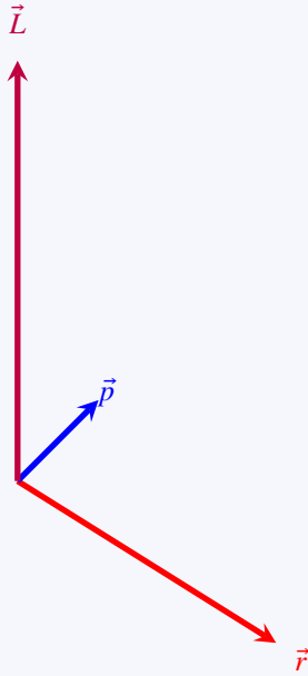
Figure 2.18 Figure of the meteor's position and momentum vectors.
