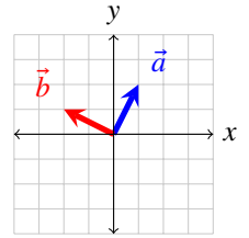
Figure 2.10 Two vectors, one rotated anti-clockwise by 90^\circ .
