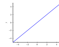
Figure 1.1 Graph of y = x .
