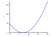
Figure 1.10 Plot of (x - 7)^2 .
