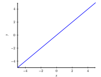
Figure 1.1: Graph of y = x .
