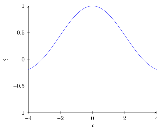
Figure 3.2 Plot of f(x) .
