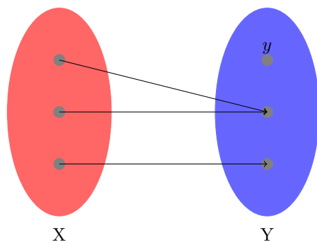
Figure 7. Illustration of non-surjective function with domain X and range Y .
