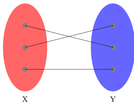
Figure 5. Illustration of an injective function with domain X and range Y .
