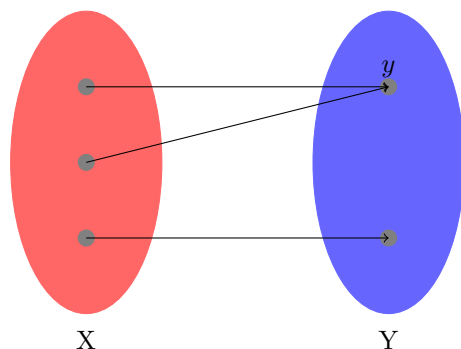
Figure 6. Illustration of a non-injective function with domain X and range Y .
