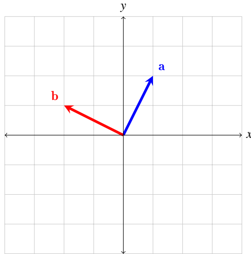
Figure 2.1 Figure of vectors a and b .
